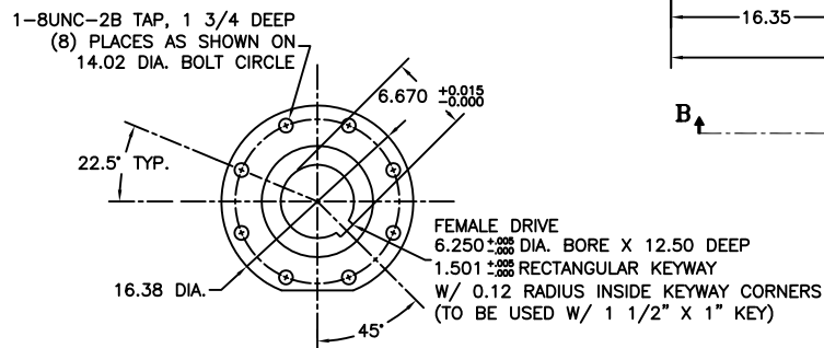
VIEW B-B ISO F35 MOUNTING PATTERN SHOWN IN CLOSED POSITION
