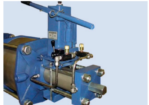
HYDRAULIC OVERRIDE - MHP
